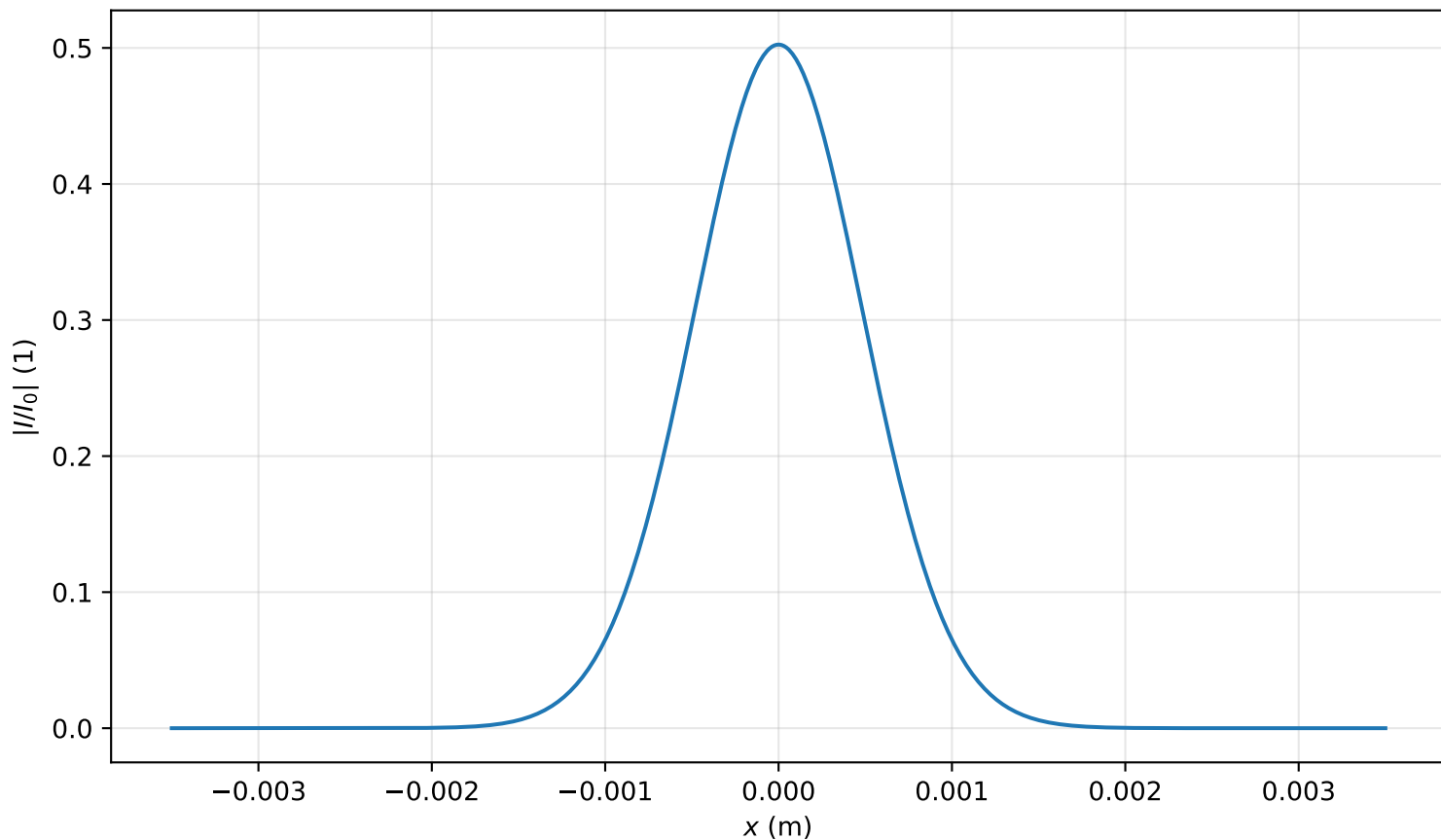
Intensity profile I(x, y = 0, z = 2.149m)/I_0 , P_{in}=0.1P_{cr} , artificial time
